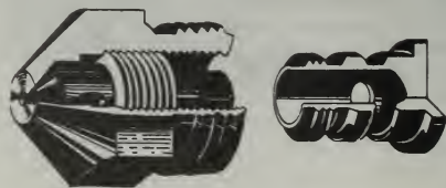
FIGURE 3-58. A typical simplex fuel nozzle.
